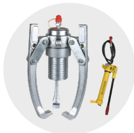
Hydraulic Remote Control Gear Puller NEX-138
